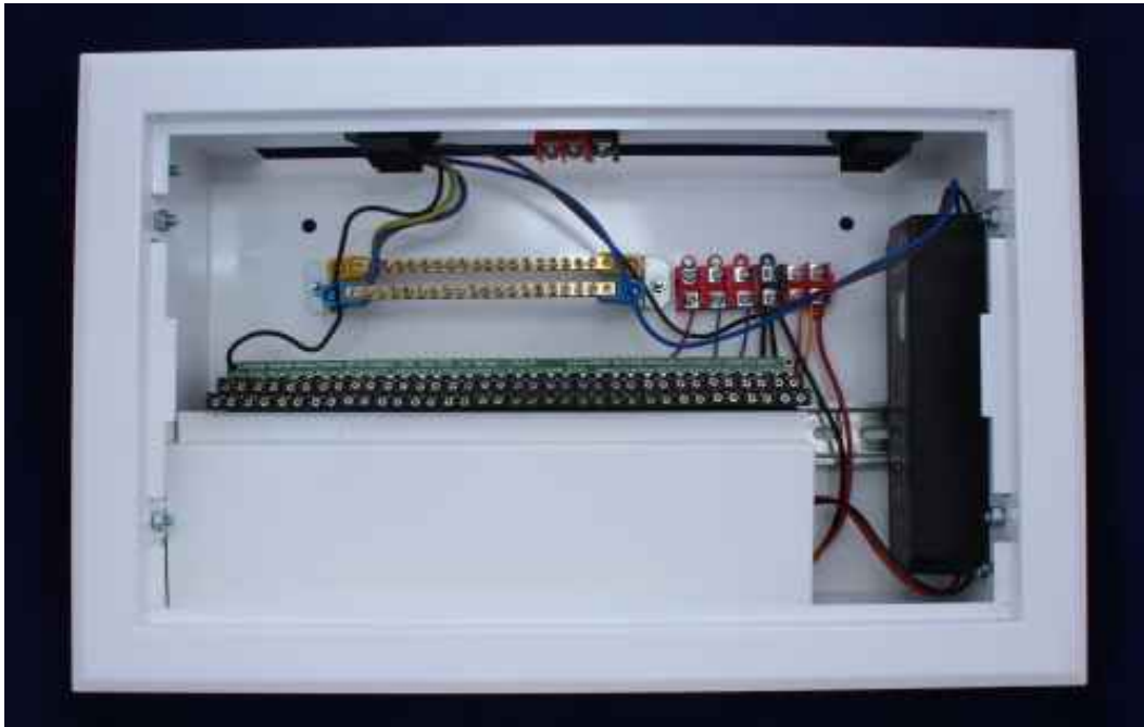
Mini-Switch board variant based on Integrated ERM+MP18 with sockets outside metal cover for easier DIY installation ( SW-MINI-ERM180-DIY )
