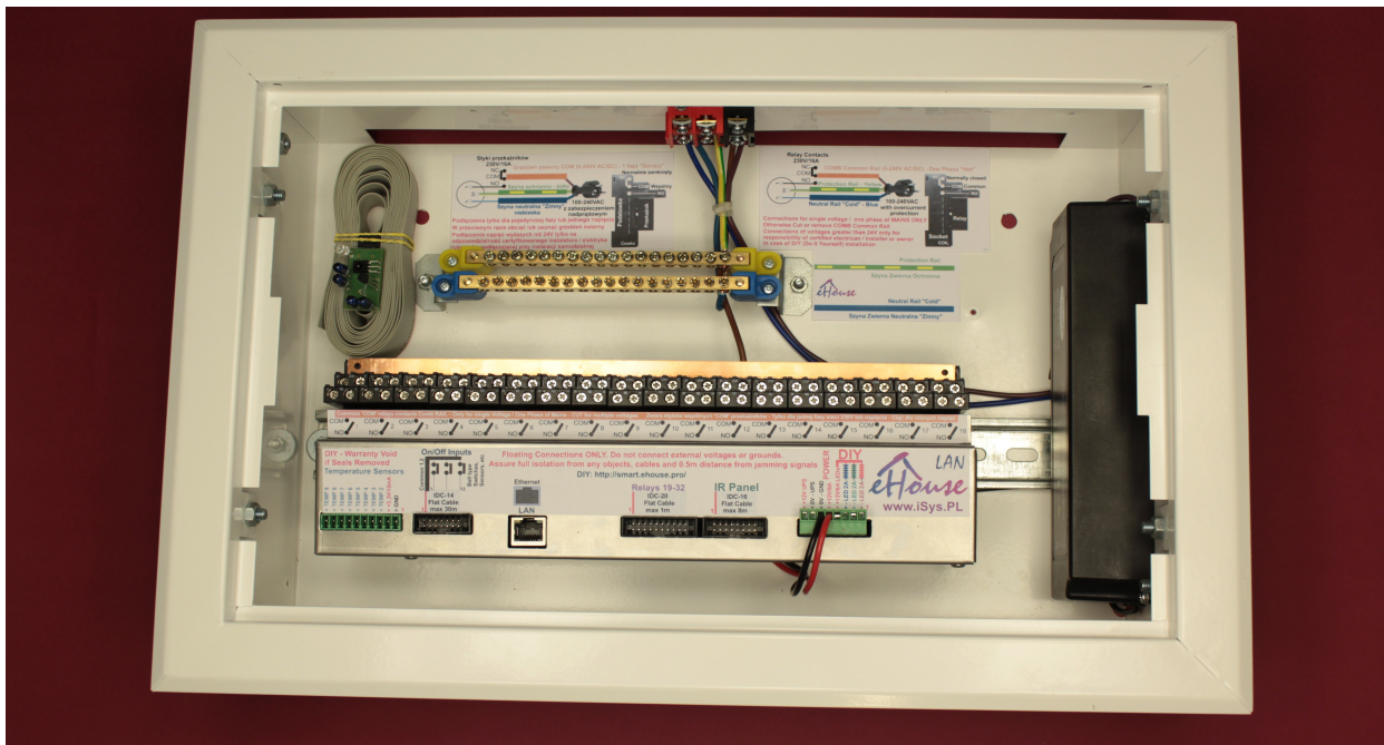
Mini-Switch board variant based on Integrated ERM+MP18 with sockets outside metal cover for easier DIY installation ( SW-MINI-ERM180-DIY )
